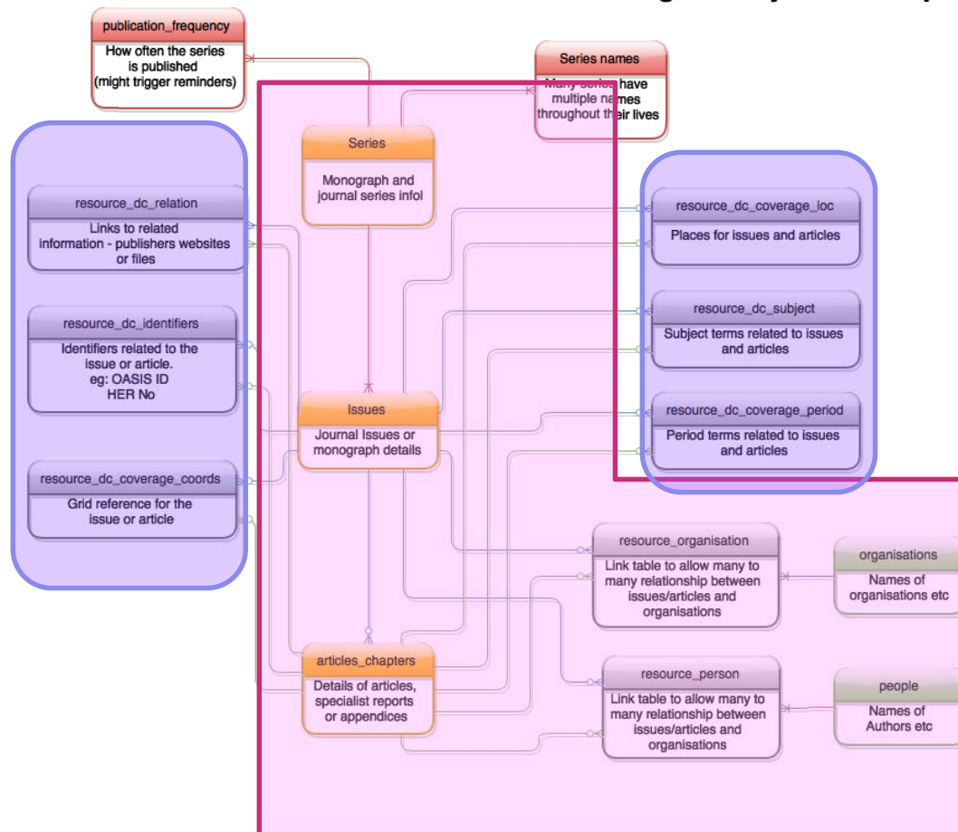
BIAB redesign - entity relationship diagram
